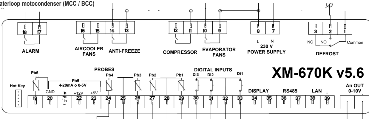
Waterloop motocondenser (MCC / BCC)
