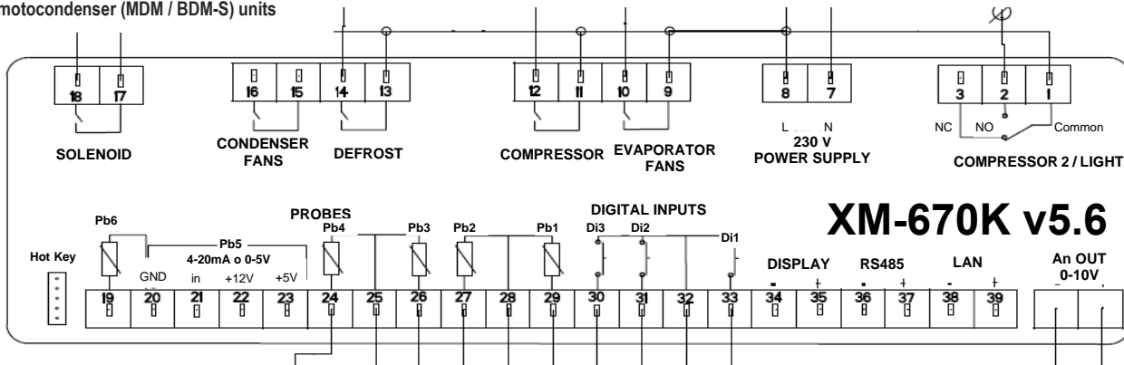
Sigilus, intarsplit, intarbox, and Waterloo motocondenser (MDM / BDM-S) units
