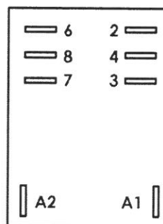
Finder Relay
