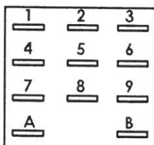
IMO Relay
